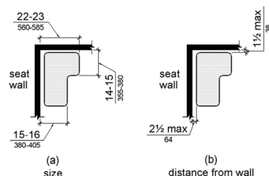
Figure 610.3.2 L-Shaped Shower Seat
