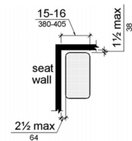
Figure 610.3.1 Rectangular Shower Seat
