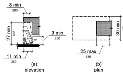
Figure 306.3 Knee Clearance
