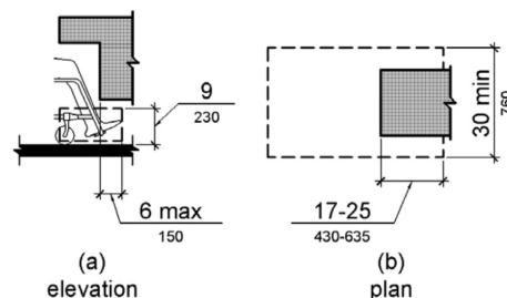
Figure 306.2 Toe Clearance
