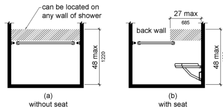
Figure 608.5.2 Standard Roll-In Type Shower Compartment Control Location
