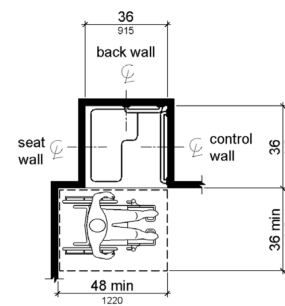
Figure 608.2.1 Transfer Type Shower Compartment Size and Clearance
