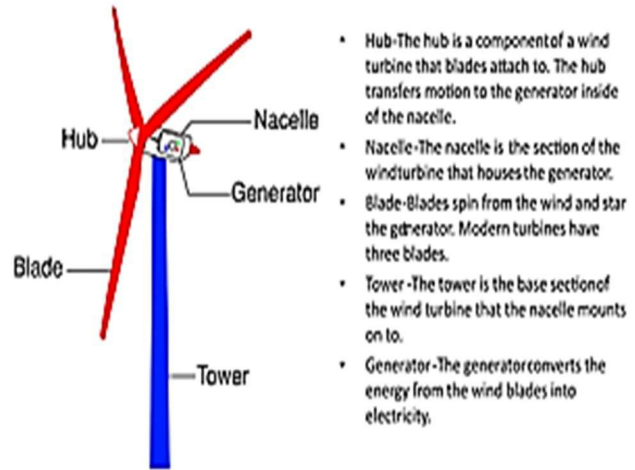
Wind Power System
