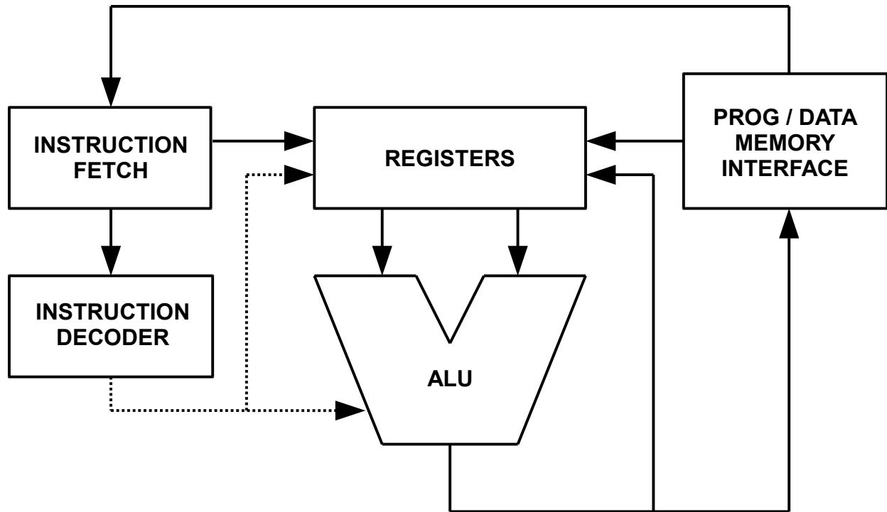
Figure 6 - Block Diagram of CPU Core
