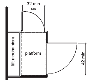
Platform Lift Doors and Gates
