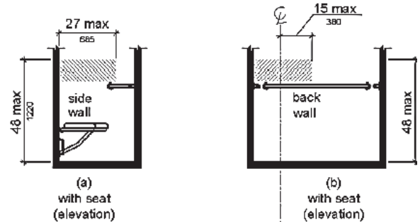
Standard Roll-In Type Shower Compartment Control Location
