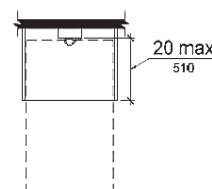
Forward Approach to Telephone
