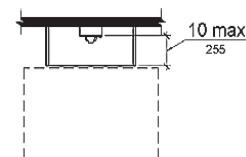
Parallel Approach to Telephone
