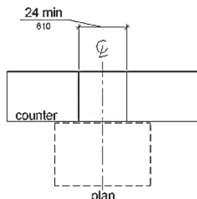
Alteration of Sales and Service Counters
