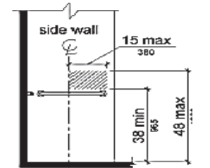
Transfer Type Shower Compartment Control Location
