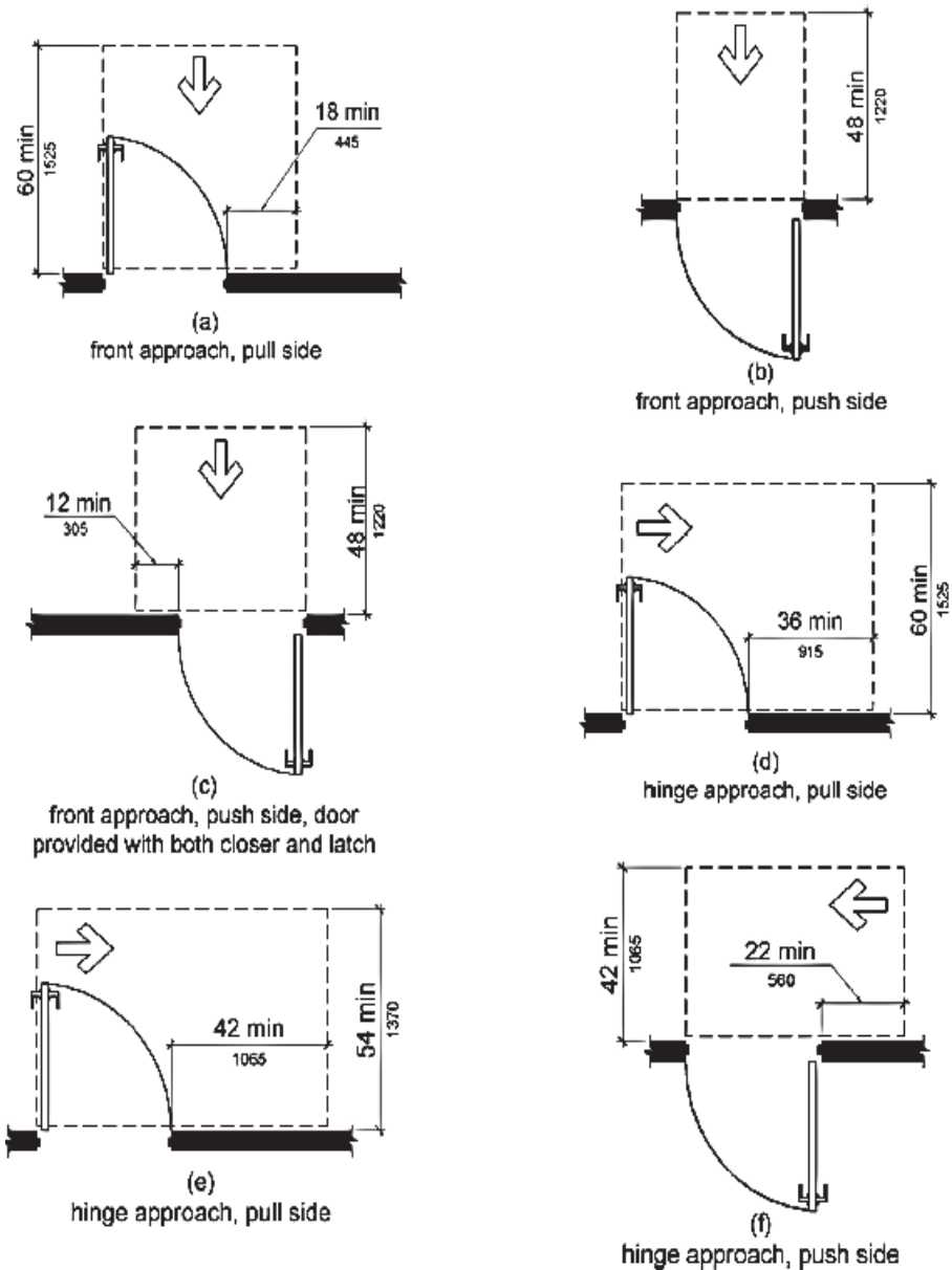
Maneuvering Clearances at Manual Swinging Doors and Gates
