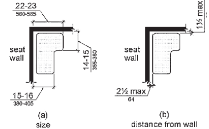
L-Shaped Shower Seat
