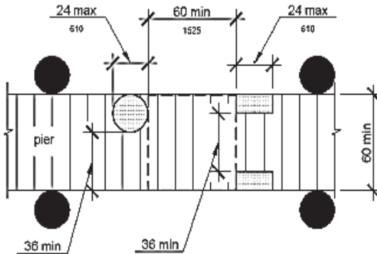
Clear Pier Space Reduction at Boarding Piers
