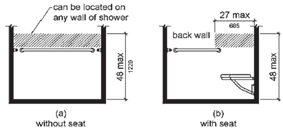
Standard Roll-In Type Shower Compartment Control Location
