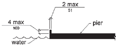
Edge Protection at Boarding Piers
