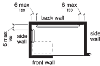
Grab Bars for Alternate Roll-In Type Showers
